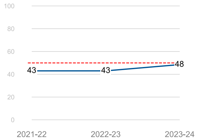
NWEA SCGP Trend
